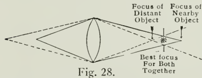
Fig. 28. Depth of Focus with Full Aperture.
